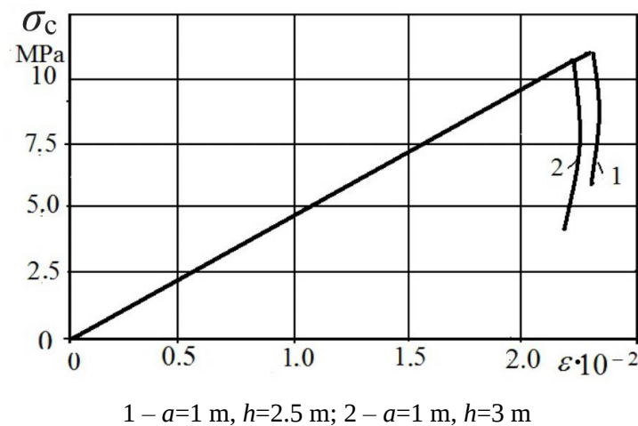
Figure 2. Diagram "stress - longitudinal strain" at the destruction of a high sample.
