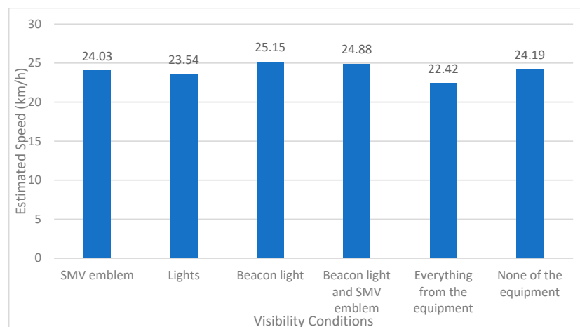
Figure 5. Descriptive statistics of the tractor's speed estimation under all tested conditions at a speed of 20 km/h.
