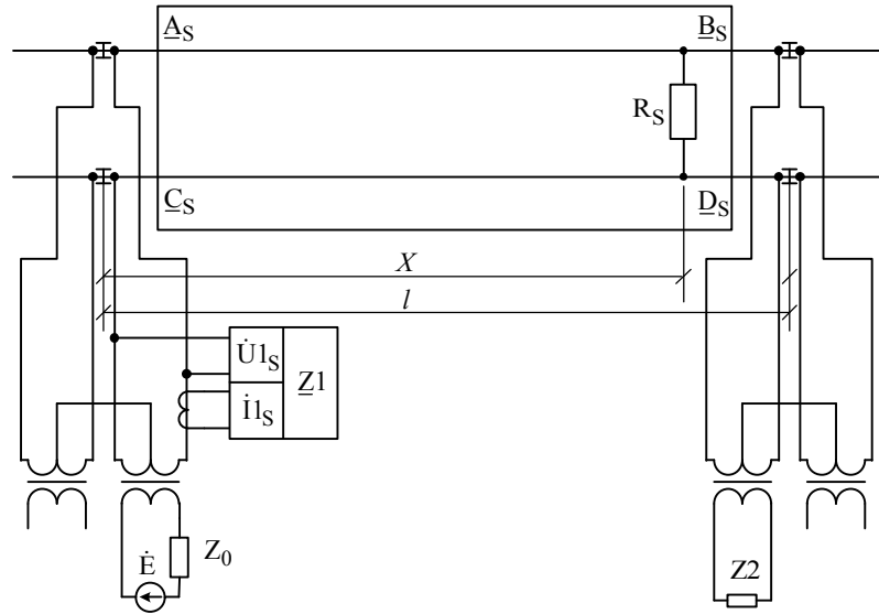
Fig. 2. The model for determining the coordinate of the shunt placement based on the track circuit input impedance.
