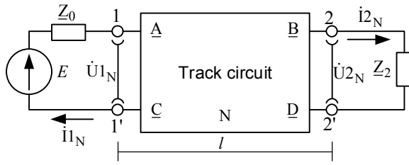
Fig. 1. Structural diagram of informative attributes measurements: \underline{Z}_0 – the complex resistance of the current limiter at the input of the track circuit, \underline{Z}_2 – the complex resistance of the load of the track circuit, \dot{U}_{1N} , \dot{I}_{1N} – respectively, the voltage and current at the input of the track circuit, \dot{U}_{2N} , \dot{I}_{2N} – respectively, the voltage and current at the output of the track circuit, N – a generalized four-pole of the entire rail line with the length l .
