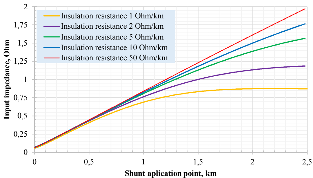
Fig. 4. Dependence of the track circuit input impedance on the shunt placement coordinate, at track circuit insulation resistances of 1, 2, 5, 10, and 50 Ohm/km.
