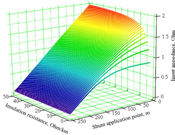
Fig. 3. Dependence of the track circuit input impedance in the shunt mode of operation on the change in insulation resistance (y-axis) and the coordinates of the shunt placement (points 1-250 – x-axis)
