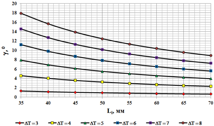
Figure 2 – Influence of parameters L_i and \Delta T on the angle of rounding of the roller by the strip: R_r = 18 mm; R_{tr} = 5.0 mm; h_s/2=2.6 mm
