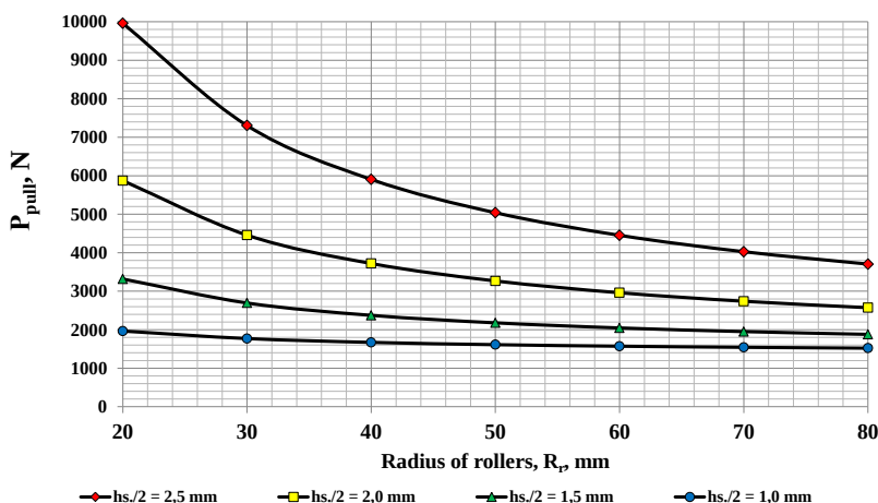
Figure 4 – The influence of the height of the strip and the radius of the rollers on the pulling force through the DBT: \sigma_{T0} = 572 N/mm 2 ; R_{cr} = 5.0 mm; L = 2R_r + 10 mm; \Delta t = 4.0 mm; n = 7 ; f = 0.01
