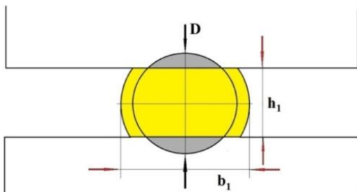
Figure 1 – Scheme of deformation of the original round workpiece in a roller die during analytical studies
