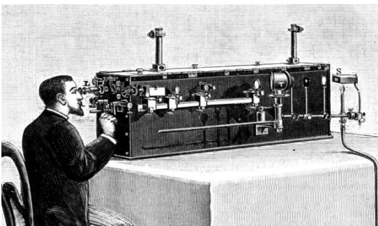
G Interferometer
