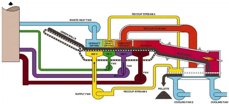
Fig. 2. Grid Installation Diagram – Tubular Kiln – Ring Cooler 20
