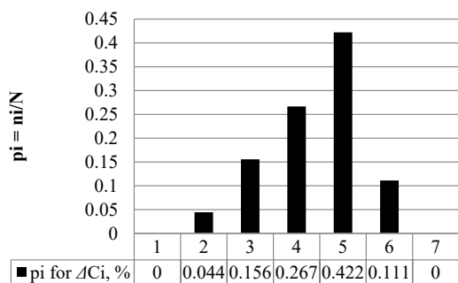
Fig. 2. Distribution of carbon content in the melt discharged from the cupola furnace: \Delta C = S_C = 0.14\% , C = 3.47 \pm 3S_C
