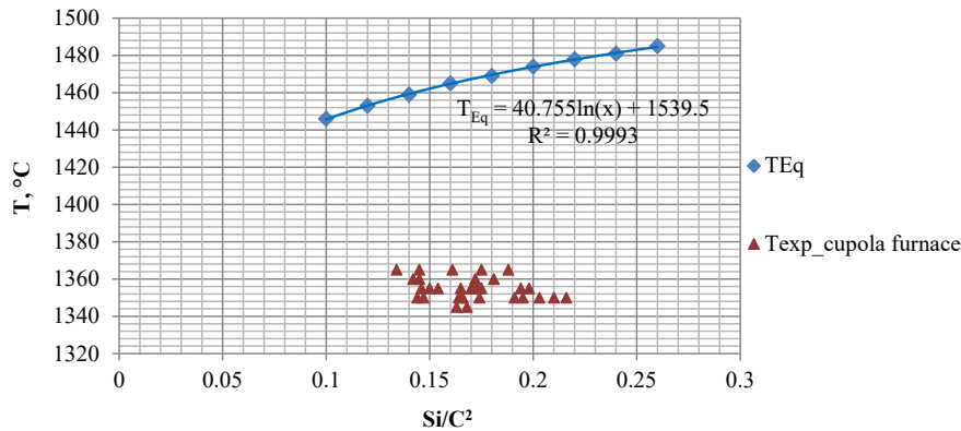
Fig. 6. The equilibrium curve of the crucible reaction and the actual indicators of the melt discharged from the cupola furnace into the induction furnace
