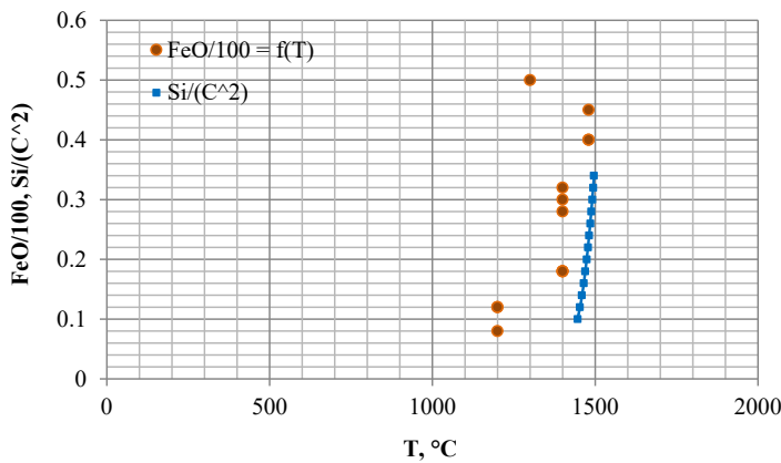
Fig. 7. Temperature regimes for removing FeO from the melt and the equilibrium curve
