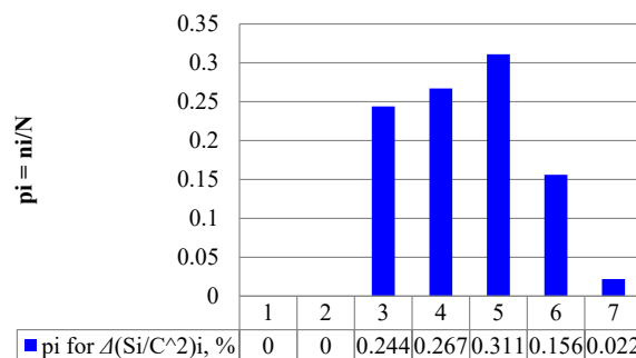
Fig. 5. Distribution histogram Si/C^2 : \Delta Si/C^2 = S_{Si/C^2} = 0.021 , Si/C^2 = 0.171 \pm 3S_{Si/C^2}
