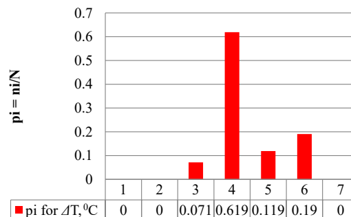
Fig. 4. Distribution of melt temperature discharged from the cupola furnace: \Delta T = S_T = 6^\circ C , T = 1355 \pm 3S_T^\circ C
