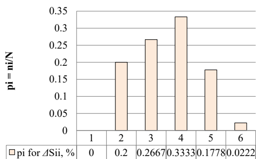
Fig. 3. Distribution of silicon content in the melt discharged from the cupola furnace: \Delta Si = S_{Si} = 0.21\% , Si = 2.05 \pm 3S_{Si}
