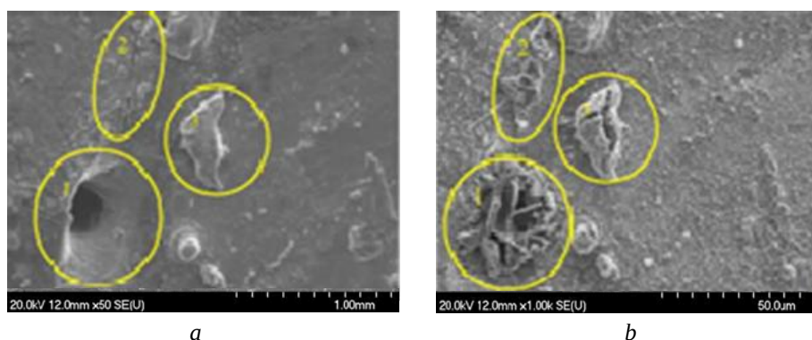
Fig. 5. SEM image of sample 2 "Position 1" in Location 2: a – before and b – after the test
