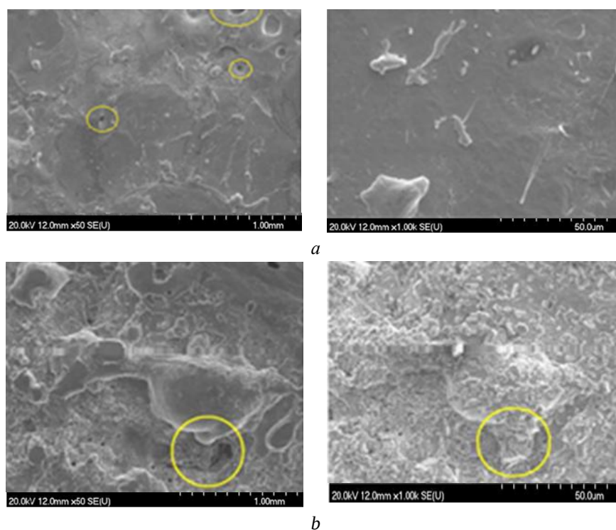
Fig. 6. SEM image of sample 3: a – before and b – after the test
