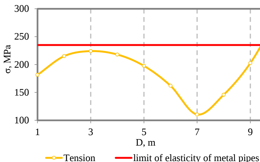
Figure 2. Dependence of the stress-strain state of the metal corrugated pipe on the structure diameter
