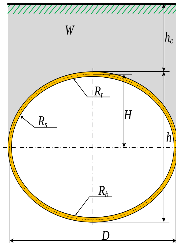
Figure 1. Geometric characteristics of the investigated metal corrugated structure
