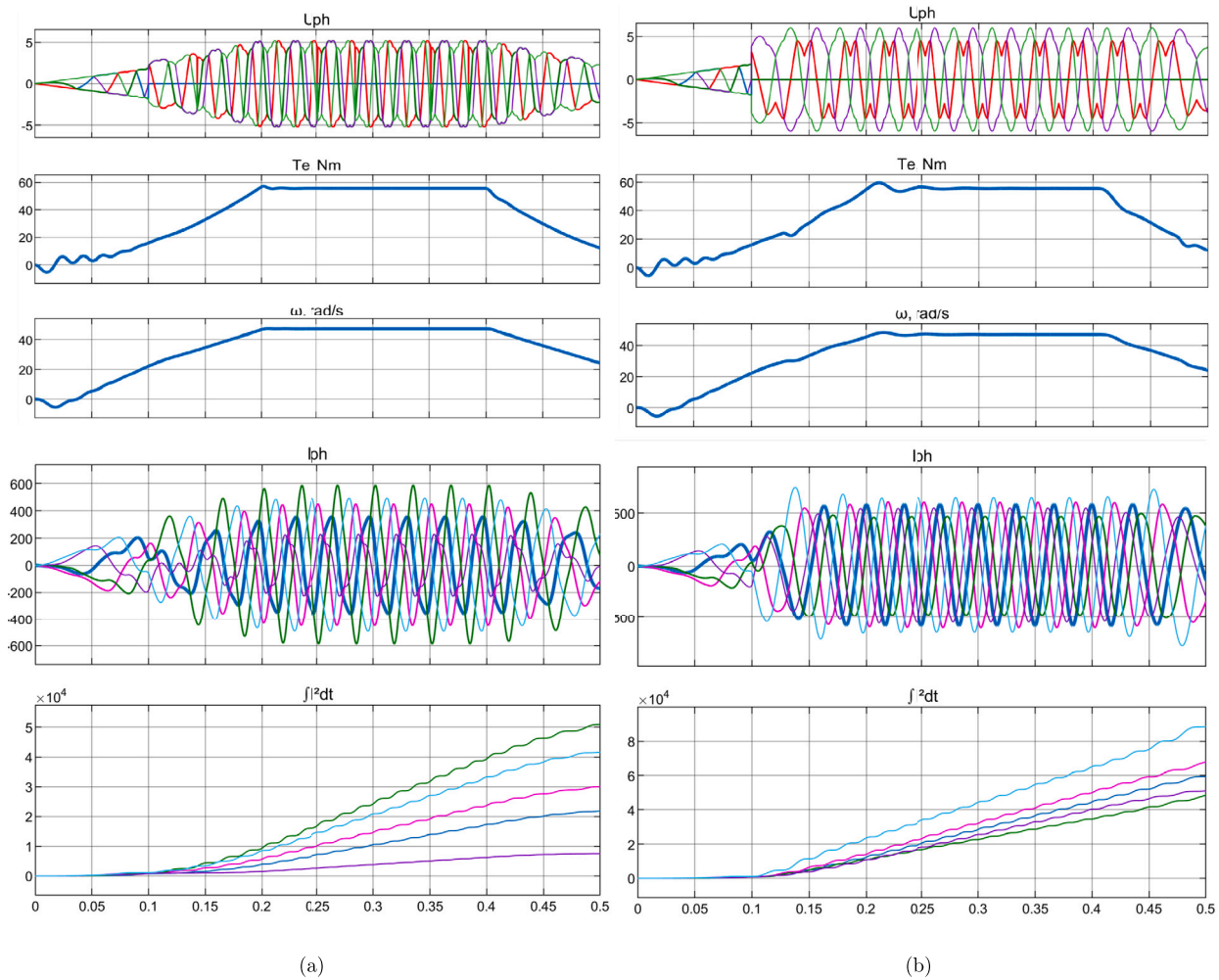
Fig. 9. Graphs of transient processes in emergency mode 0-6-6-6-6 (a) and 0-6-0-6-6 (b).
