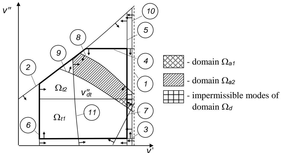
Fig. 3. Selection of domain of permissible braking modes
